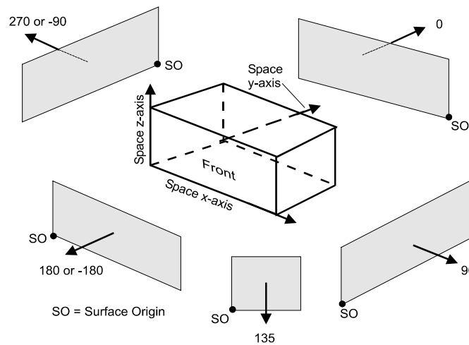
Figure 8 Examples of Wall Azimuth Values
