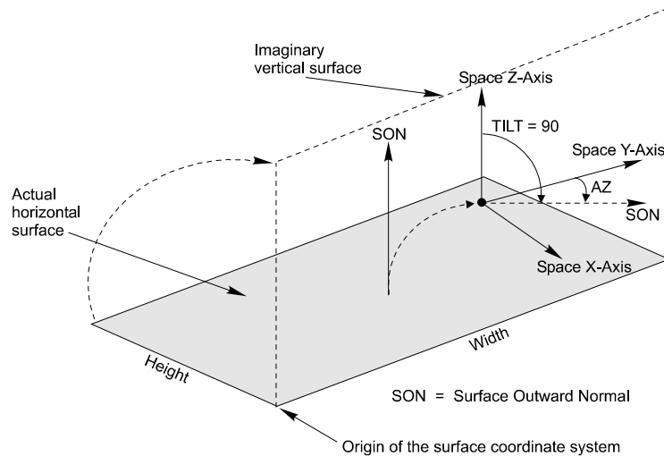
Figure 9 Method of describing a Horizontal Surface
