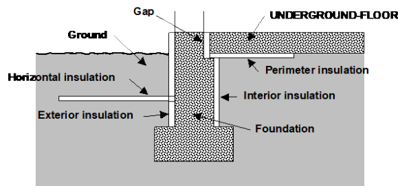
Figure 23 Slab-on-Grade
