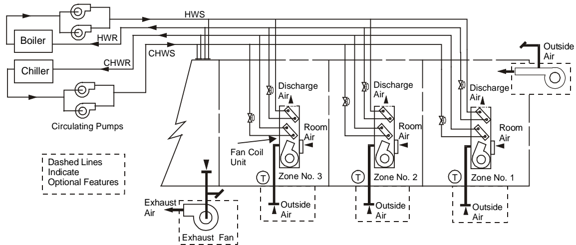
Figure 56 Four-pipe fan coil system
