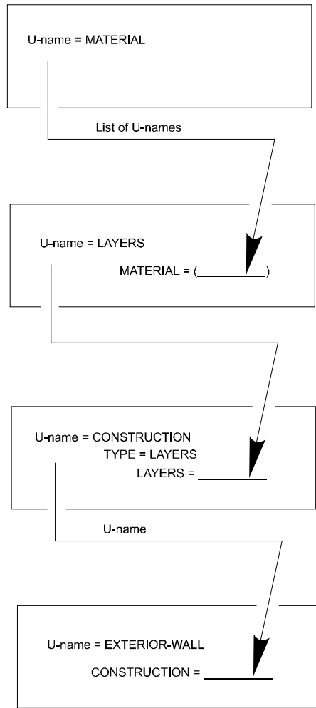
Figure 19 Specifying a "delayed" EXTERIOR-WALL (without a library)
